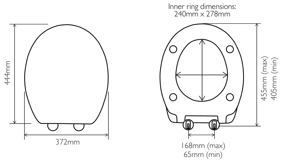
General seat dimensions
