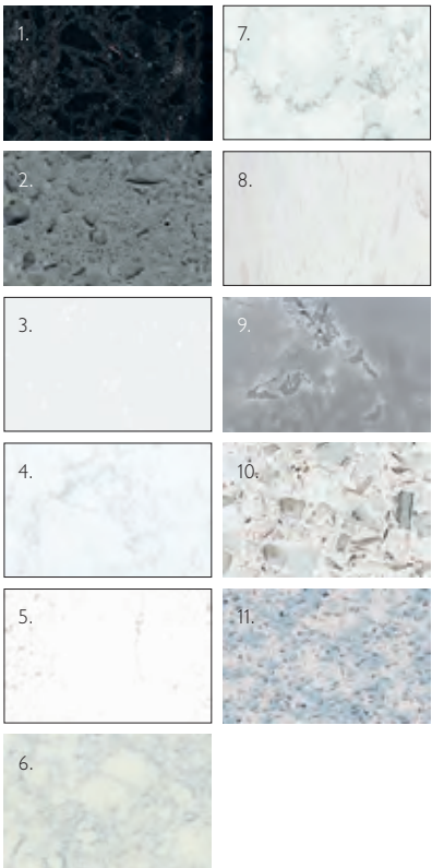
Image shows quartz in Vesta.
