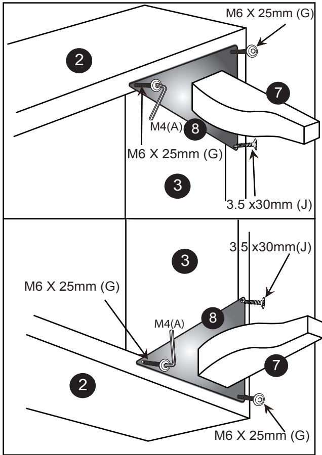
For Footboard
